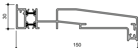
AW542 150mm Cill
