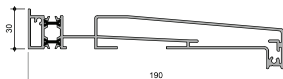
AW544 190mm Cill
