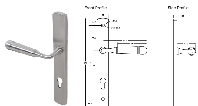
Opera Lever Door Handle on Backplate- TBH095
