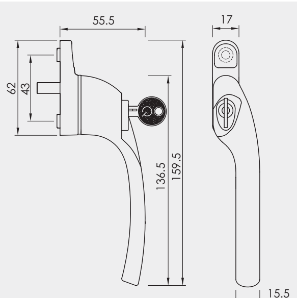
Alpha Right Crank Espag Handle with Cylinder
