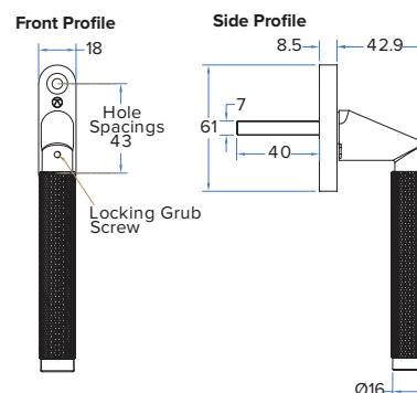
Newton Knurled Inline Window Espag Handle - NTN340
